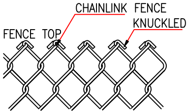
CHAINLINK FENCE BOTH SIDES KNUCKLED
